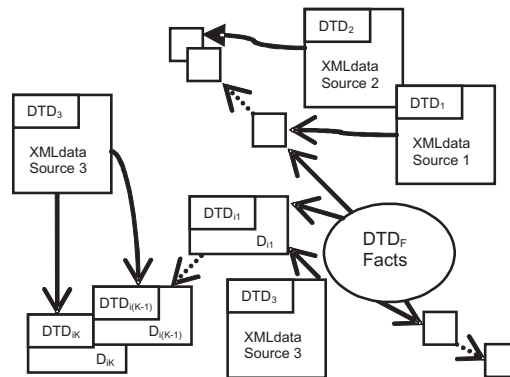
Figure 2.5: XML-star schema [66]
