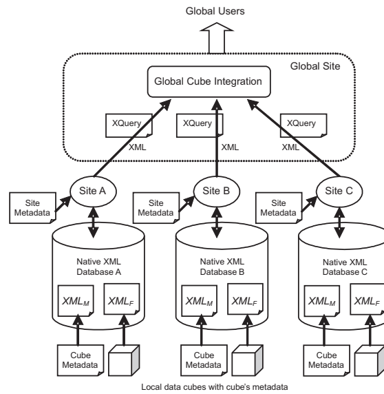
Figure 2.3: Federated DW architecture [84]
