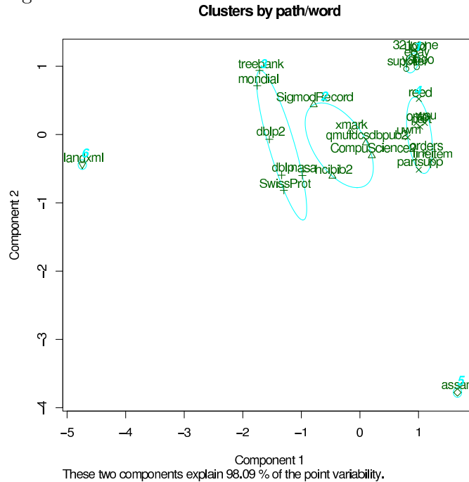
Figure 2.16: Clustering collections by heterogeneity characteristics, including two highly heterogeneous collections.
